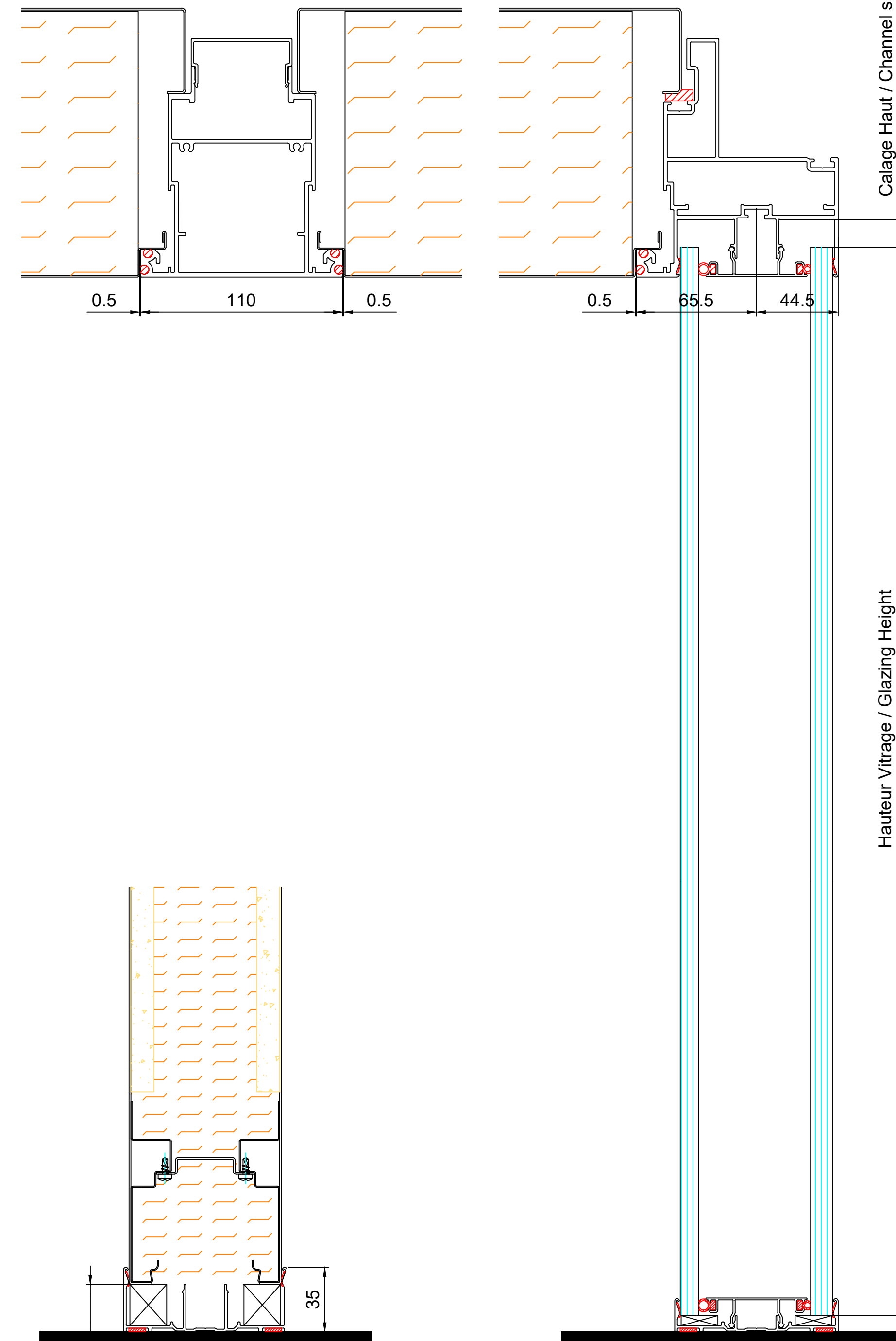
SECTION B-B
