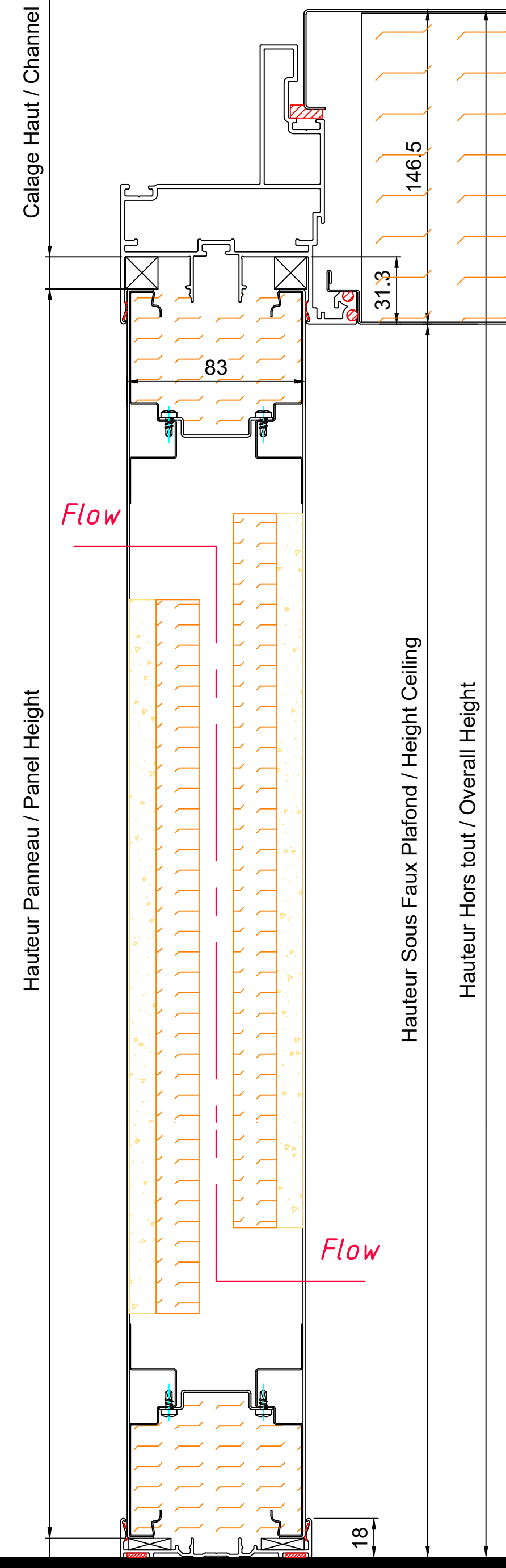
SECTION B-B
